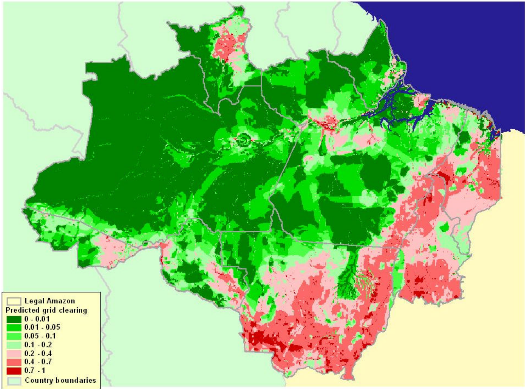
Figure 16. Prediction based on the disaggregation technique
