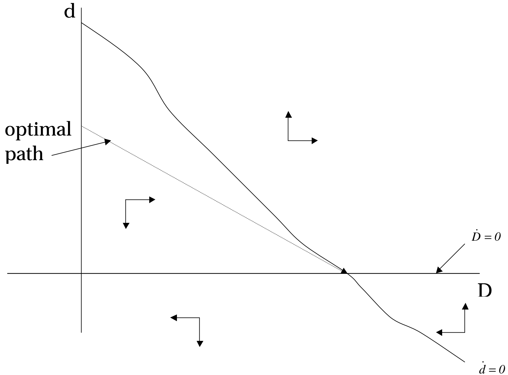
Figure 12. Phase plane diagram assuming concave production function
